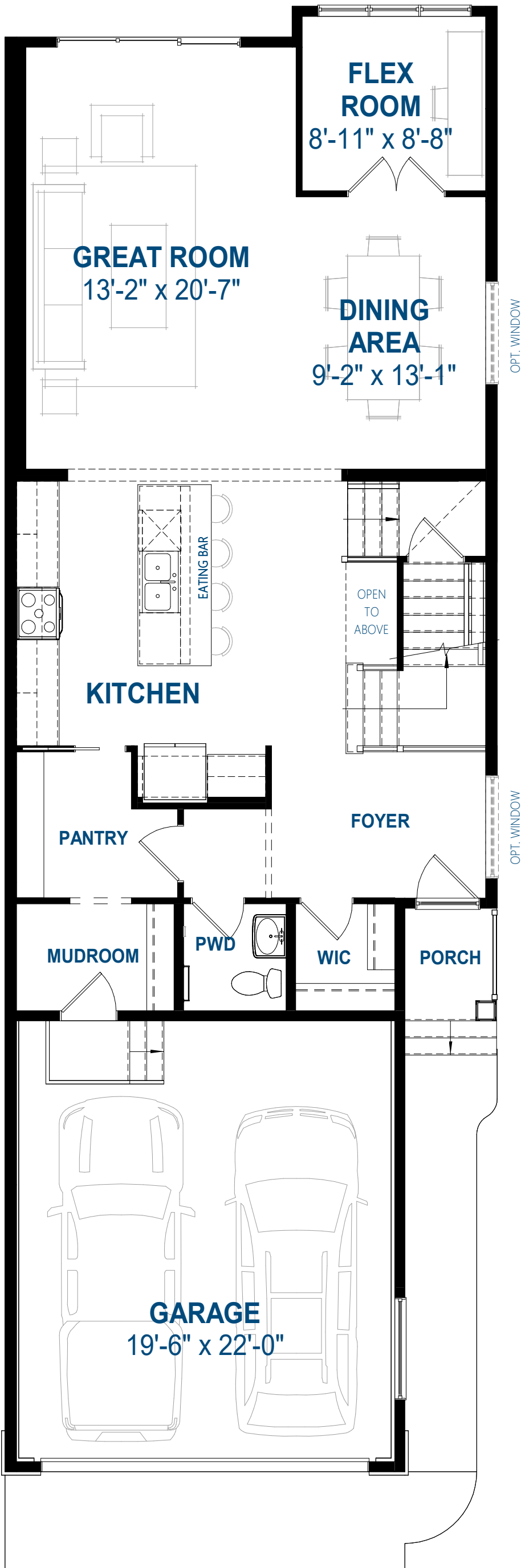
MAIN FLOOR STANDARD (1143 SQ. FT.)
